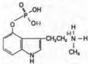
BAEOCYSTIN
